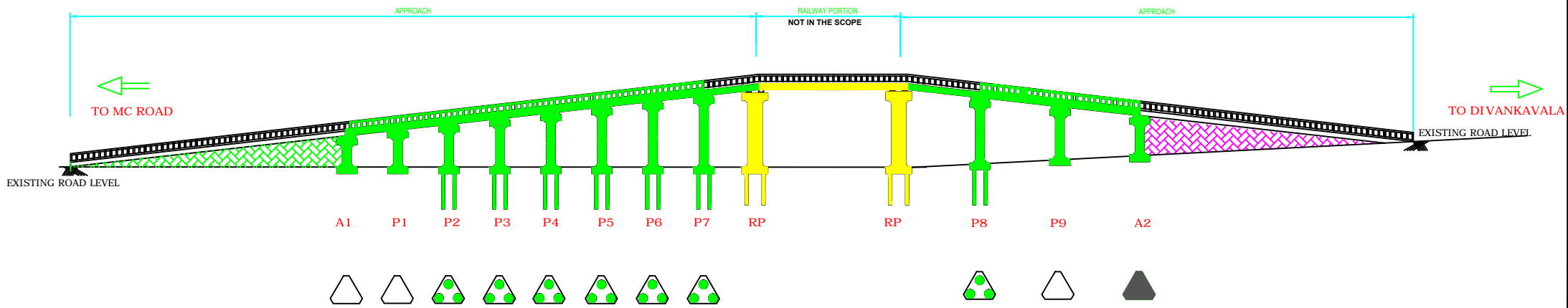
PILE FOUNDATION
